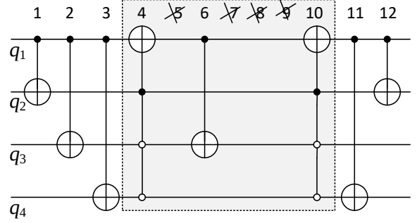
Figure 9. Reduced quantum circuit for V_3 \cdot V_4
