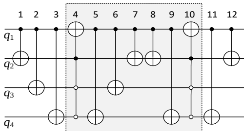
Figure 8. Quantum circuit for matrix V_3 \cdot V_4
