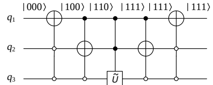
Figure 4. Non-trivial operation of U on |000\rangle
