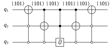
Figure 3. Trivial operation of U on |101\rangle
