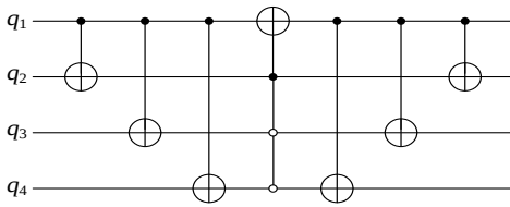
Figure 7. Quantum circuit for matrix V_4 The quantum circuit for V_3 \cdot V_4 is then as follows:
