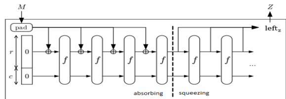
Fig.1. The Sponge construction
