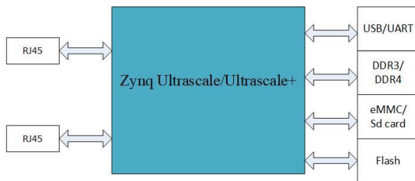
Figure 10. Block diagram of the Gateway mode IP network security device design using FPGA technology integrated with ARM platform
